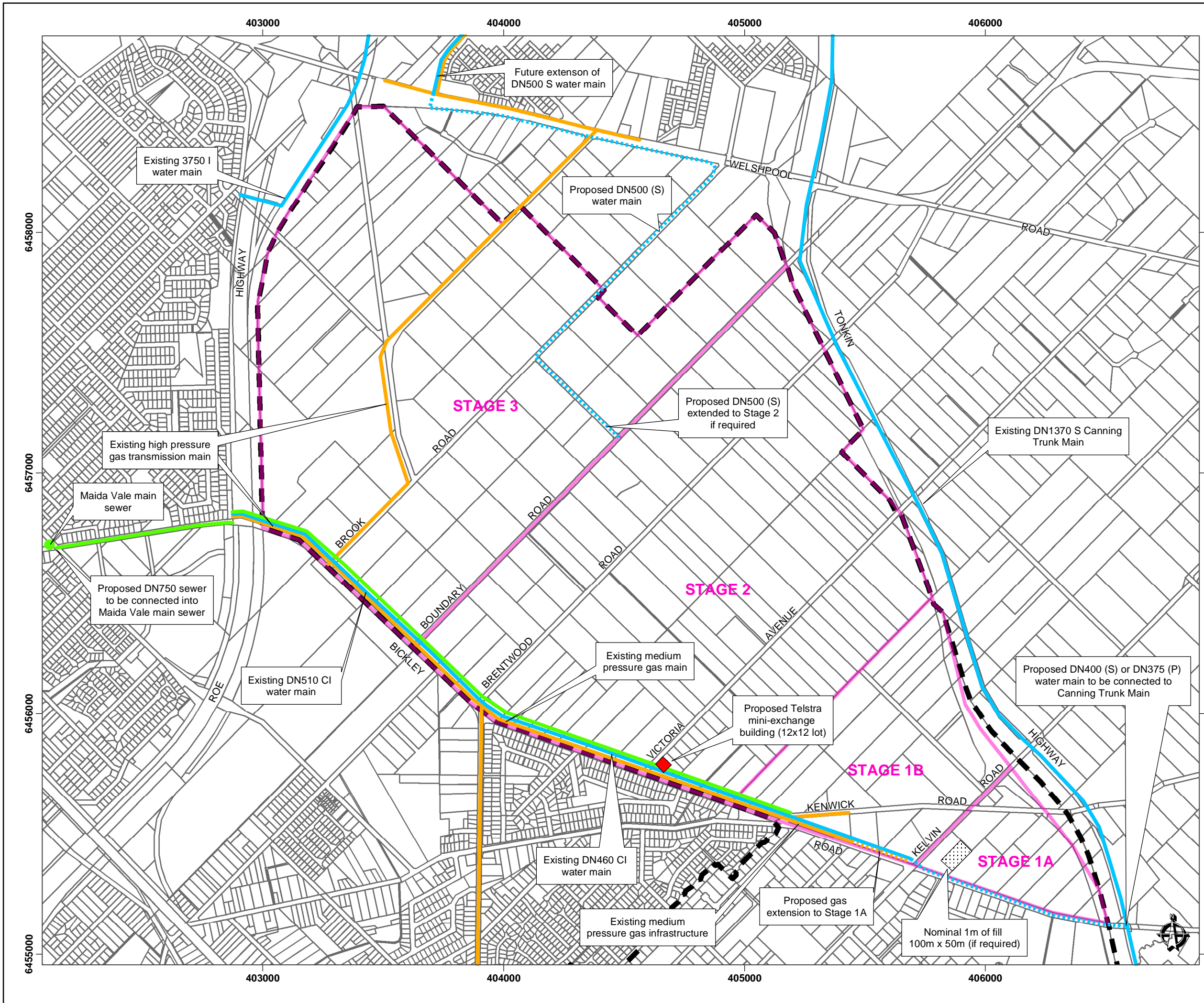
Figure 10 Trunk Main Infrastructure Plan
