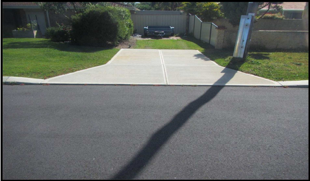
Figure 3 - Concrete crossing - Compliant
