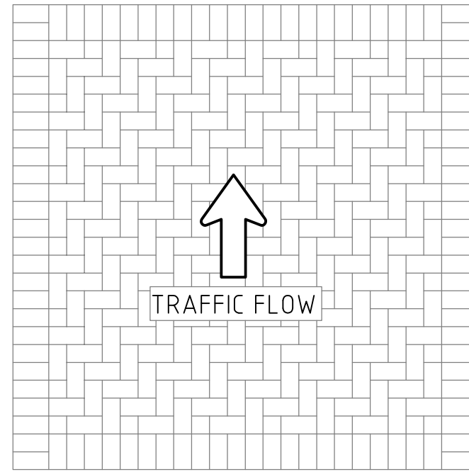
90° HERRINGBONE
